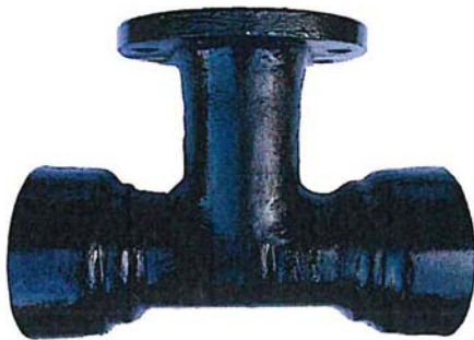
Double Socket Tees with Flanged Branch
