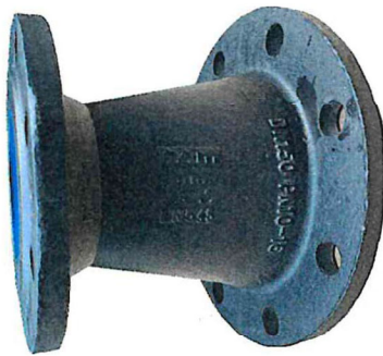
Double Flange Concentric Taper
