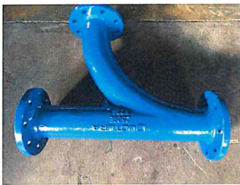
All Flanged Radial Tees PN25
