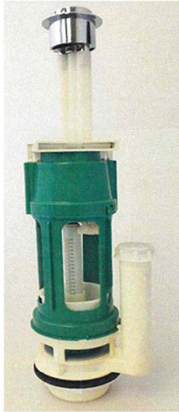
Dudley Niagara Mechanical Dual Flush Valve
