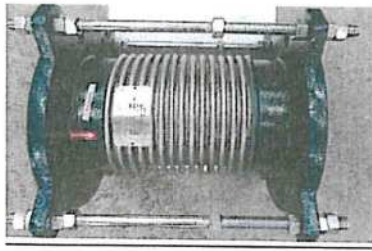
JF-150SG/SS316
