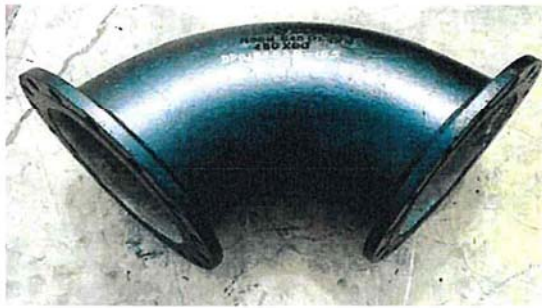
Double Flanged 90° Bend
