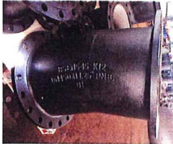
Double Flanged 11.25° Bend
