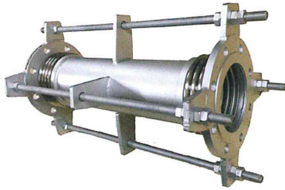
JBU-316P
