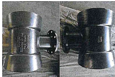
Double Socket Tee with Flange Branch PN16
