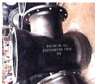
Double Socket Tee with Flange Branch
