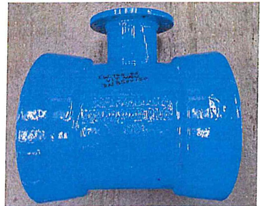
Double Socket Invert Tee with Flanged Branch
