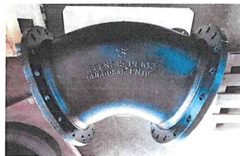
Double Flanged 45° Bend
