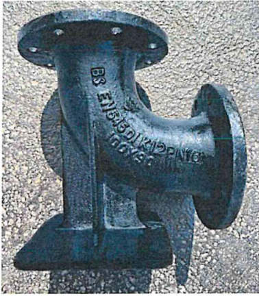
Double Flanged 90° Duckfoot Bend
