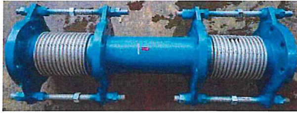
JF-850SG(PN25)
