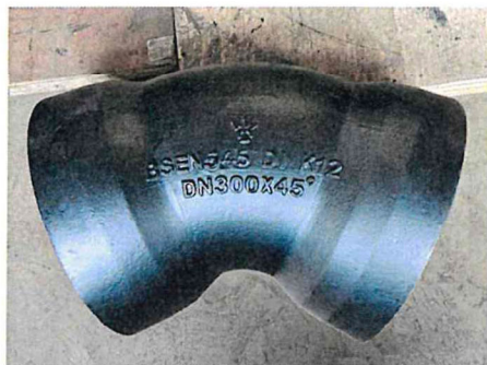
Double Socket 45° Bend
