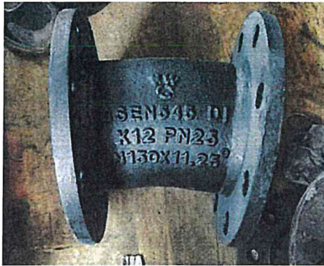
Double Flanged 11.25° Bend
