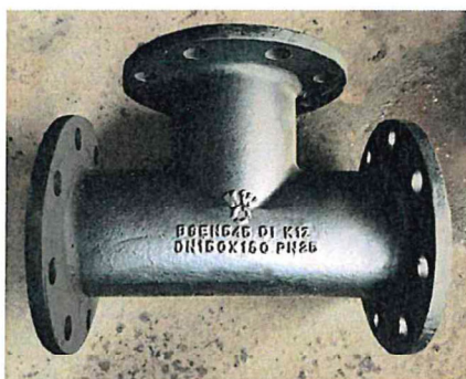
All Flanged Tee
