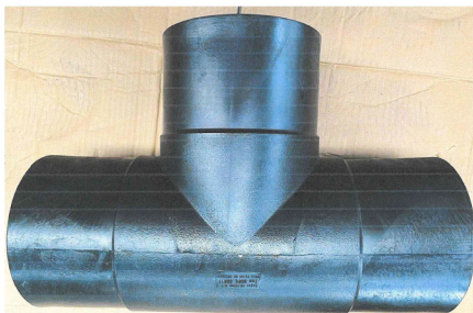
Spigot Equal Tee
