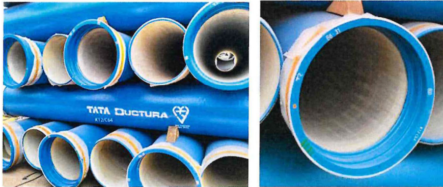
Ductile iron pipes with push in flexible joints (Class C)
