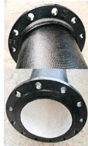
Ductile iron pipes with screw-on flanged (Class C)
