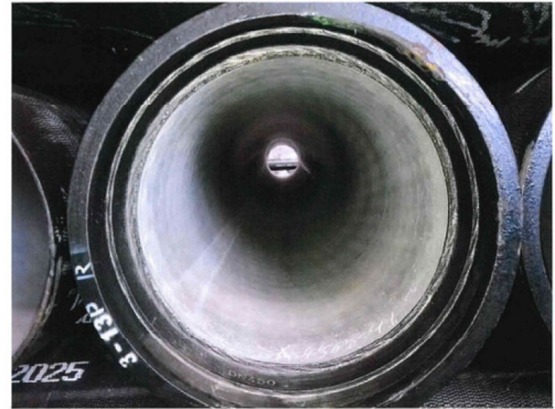
Ductile iron socket and spigot pipes (Class C)
