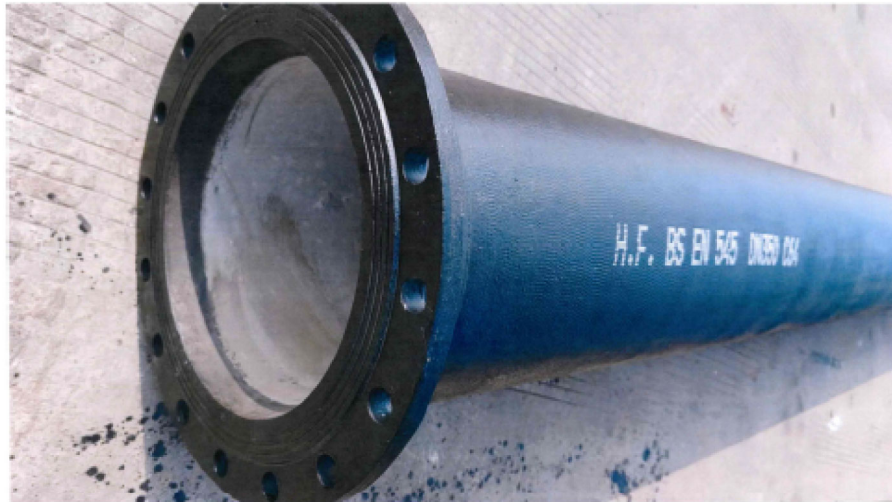
Ductile iron pipes with welded-on flanged (Class C)
